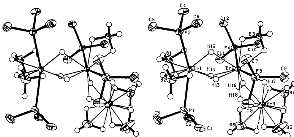
Figure 3. Stereoview of the molecular structure of Zr_3H_6(BH_4)_6(PMe_3)_4 , 1 , showing the 35% probability surfaces. The hydrogen atoms are represented by arbitrarily-sized spheres.
