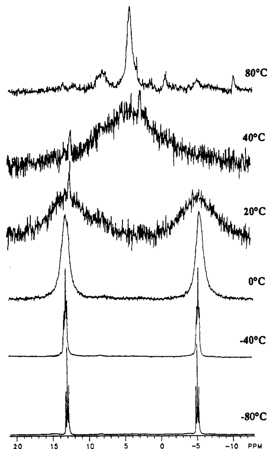
Figure 9. Variable-temperature 121.5-MHz ^{31}\text{P}\{^1\text{H}\} NMR spectrum of \text{Hf}_2\text{H}_4(\text{BH}_4)_4(\text{dmpe})_2 , 4 , in \text{C}_7\text{D}_8 . Some decomposition is evident at 80 ^\circ\text{C} .
