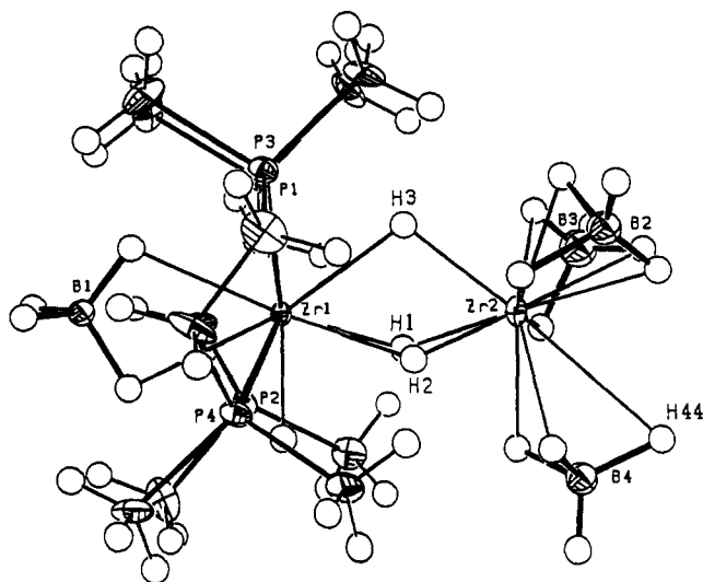
Figure 7. ORTEP diagram of Zr_2H_4(BH_4)_4(dmpe)_2 , 3, rotated 90^\circ from the view in Figure 7, showing lengthening of the Zr(2)-H(44) bond.
