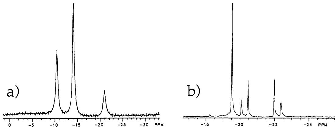
Figure 2. Heteronuclear NMR spectra of Zr_3H_6(BH_4)_6(PMe_3)_4 , 1 , in C_7D_8 : (a) 96.3-MHz ^{11}B\{^1H\} NMR spectrum at 20 °C and (b) 121.5-MHz ^{31}P\{^1H\} NMR spectrum at -80 °C.
